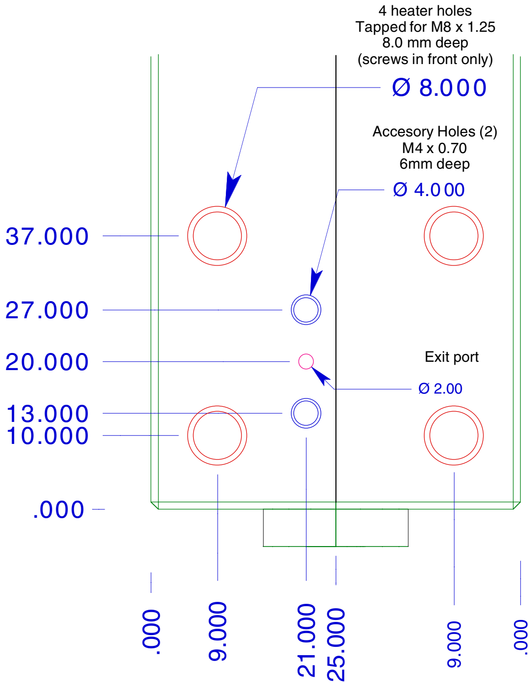
DACA Instruments MicroCompounder exit port All dimensions in mm
